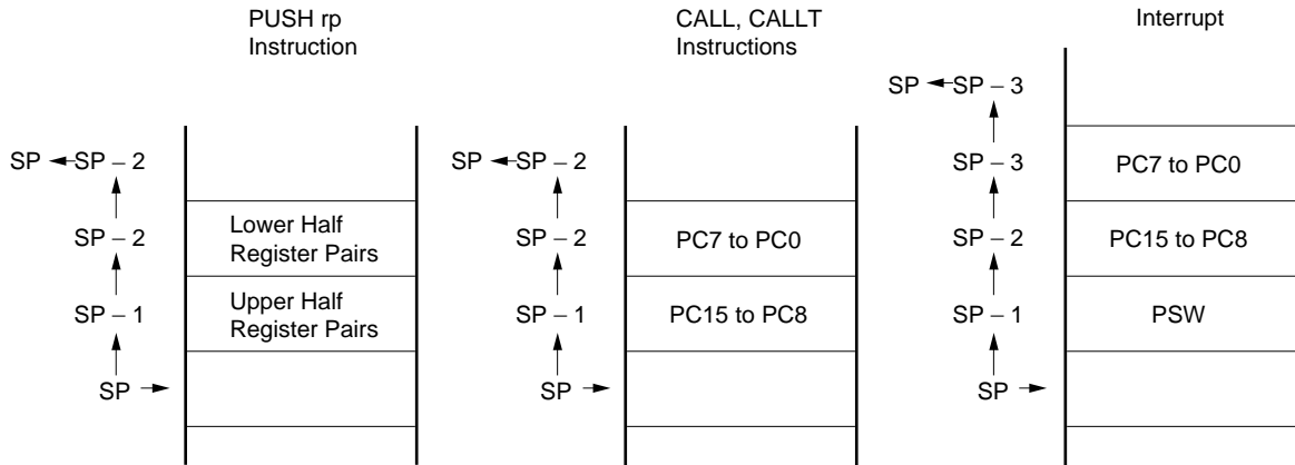
Figure 3-14. Data to be Saved to Stack Memory
